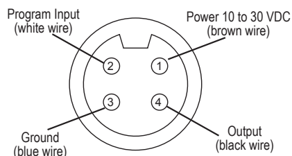
Connector View
